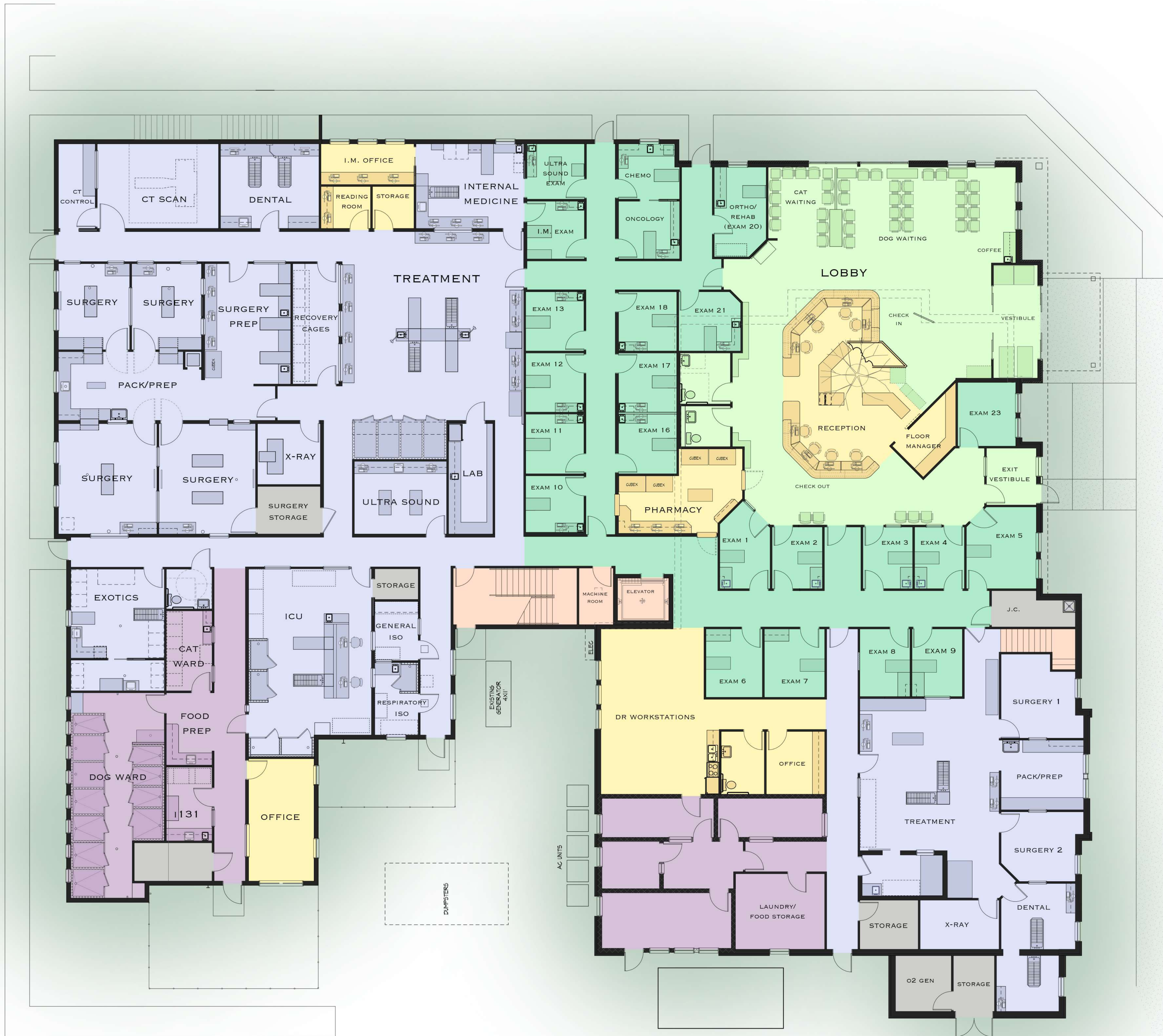
MT LAUREL ANIMAL HOSPITAL PROPOSED FIRST FLOOR PLAN 9/11/2017
